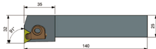
MTFNR-2525M16 牌價：MCKNR-25
