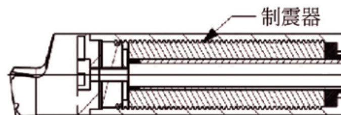
Monkula anti-vibration cutters
